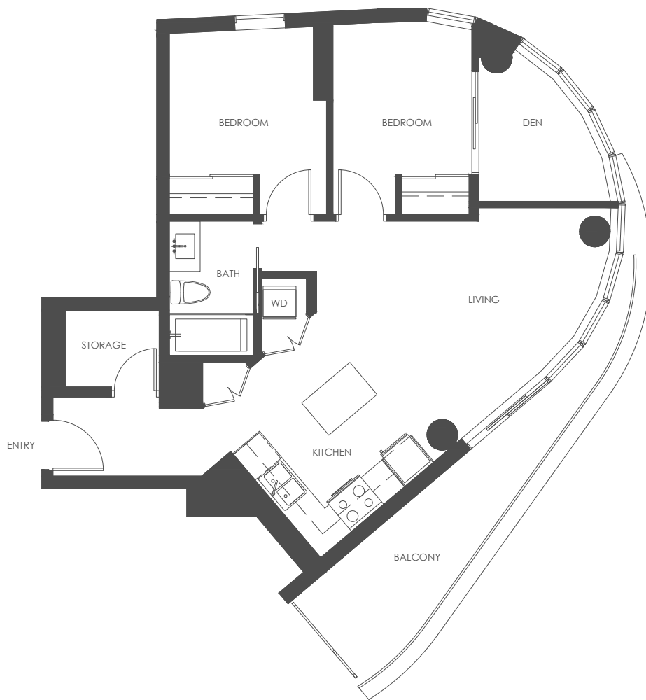
TYPICAL FLOOR
